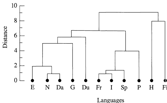
Figure 12.10 Average linkage dendrogram for distances between numbers in 11 languages.
