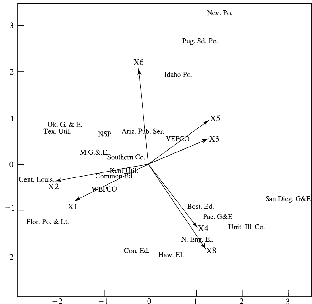
Figure 12.22 A biplot of the data on public utilities.
