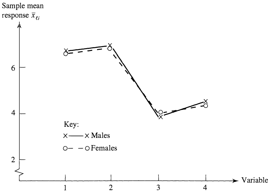
Figure 6.5 Sample profiles for marriage-love responses.
