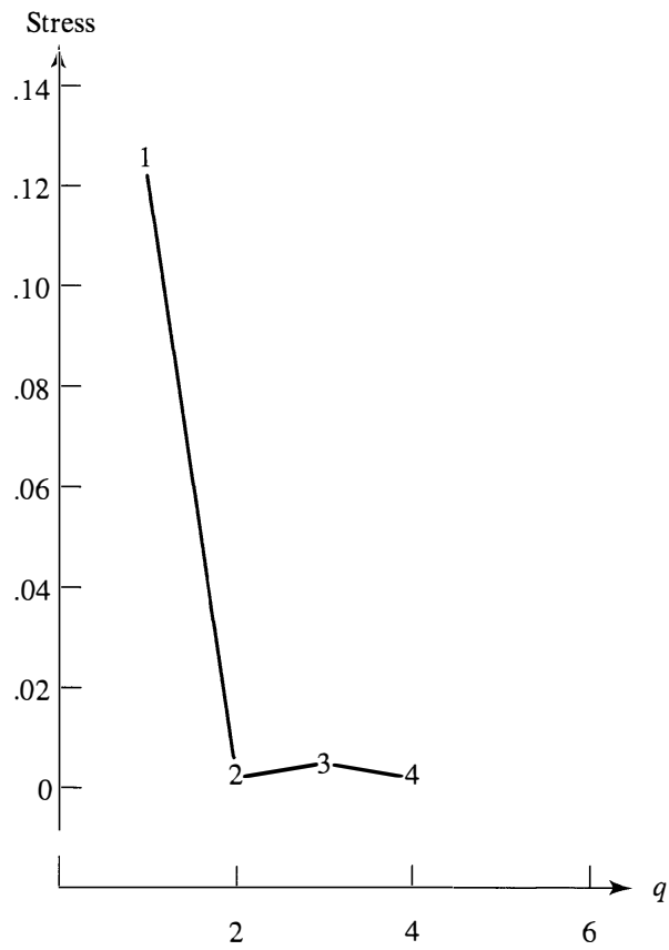
Figure 12.15 Stress function for airline distances between cities.
