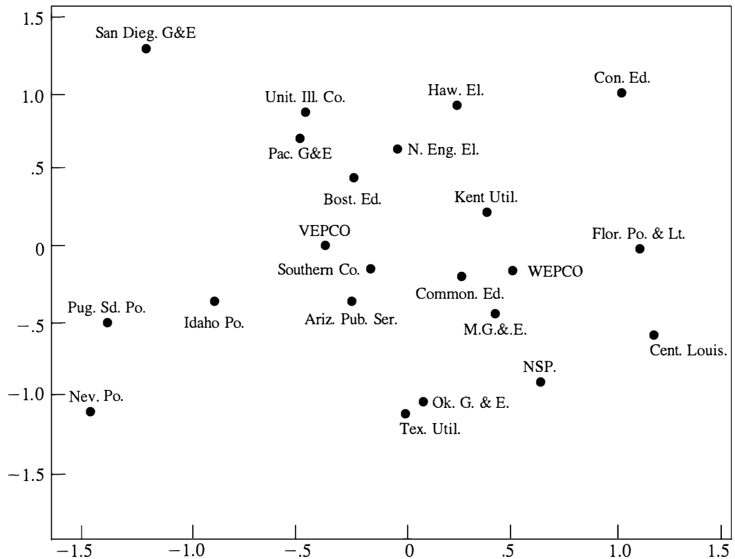
Figure 12.17 A geometrical representation of utilities produced by multidimensional scaling.
