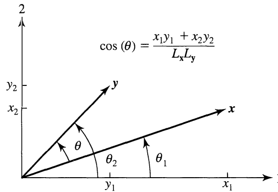
Figure 2.4 The angle \theta between \mathbf{x}' = [x_1, x_2] and \mathbf{y}' = [y_1, y_2] .
