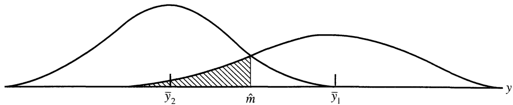
Figure 11.7 Schematic of normal densities for linear discriminant—salmon data.
