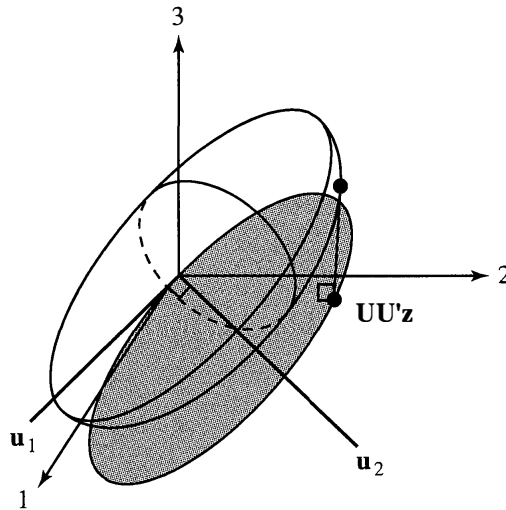
Figure 5.13 The shadow of the ellipsoid \mathbf{z}' \mathbf{A}^{-1} \mathbf{z} \leq c^2 on the \mathbf{u}_1, \mathbf{u}_2 plane is an ellipse.
