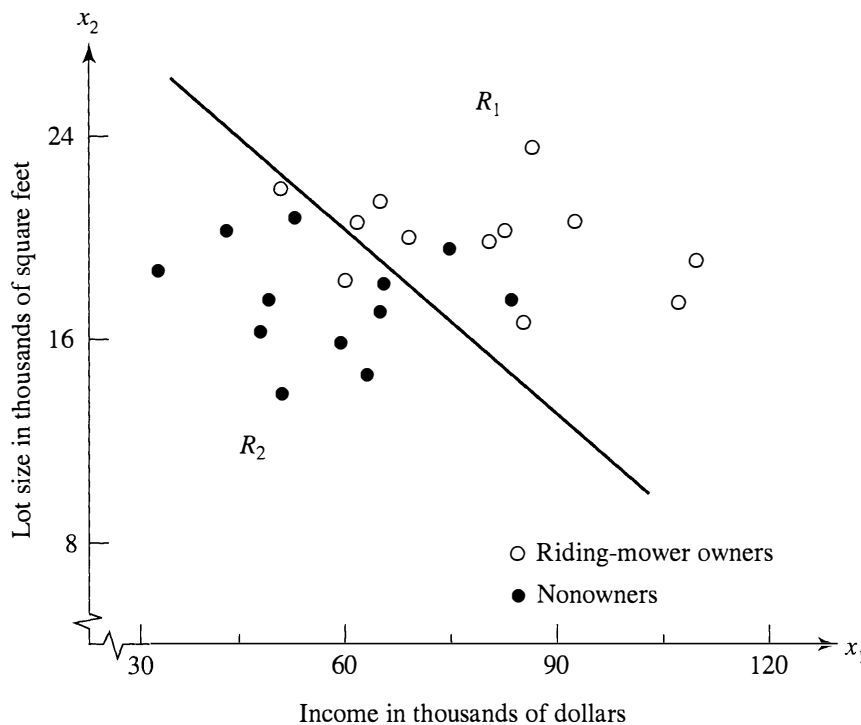
Figure 11.1 Income and lot size for riding-mower owners and nonowners.
