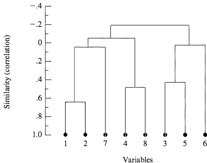
Figure 12.9 Complete linkage dendrogram for similarities among eight utility company variables.
