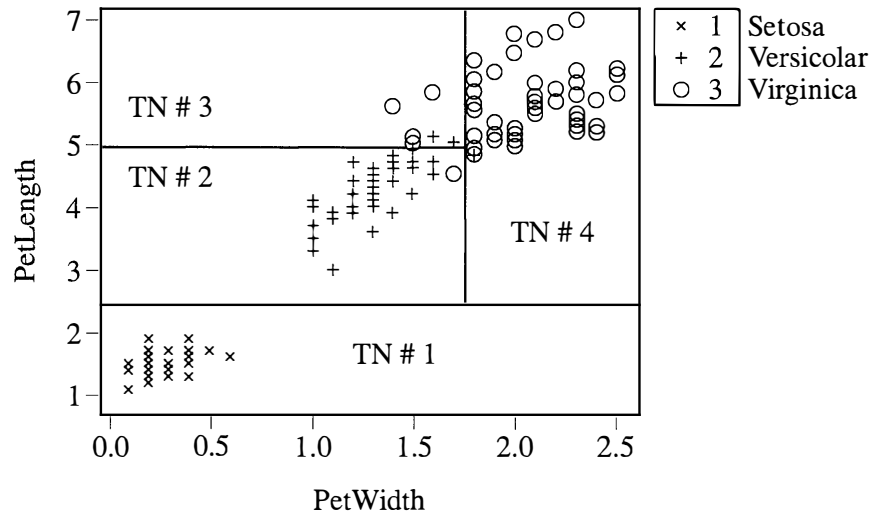
Figure 11.17 Classification tree terminal nodes (regions) in the petal width, petal length sample space.
