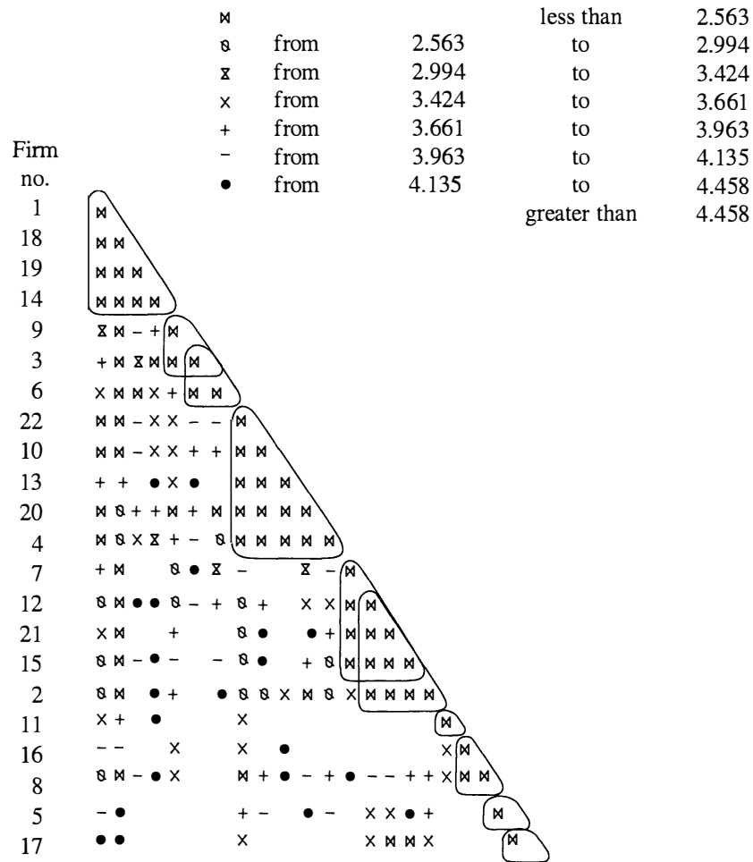
Figure 12.2 Shaded distance matrix for 22 utilities.
