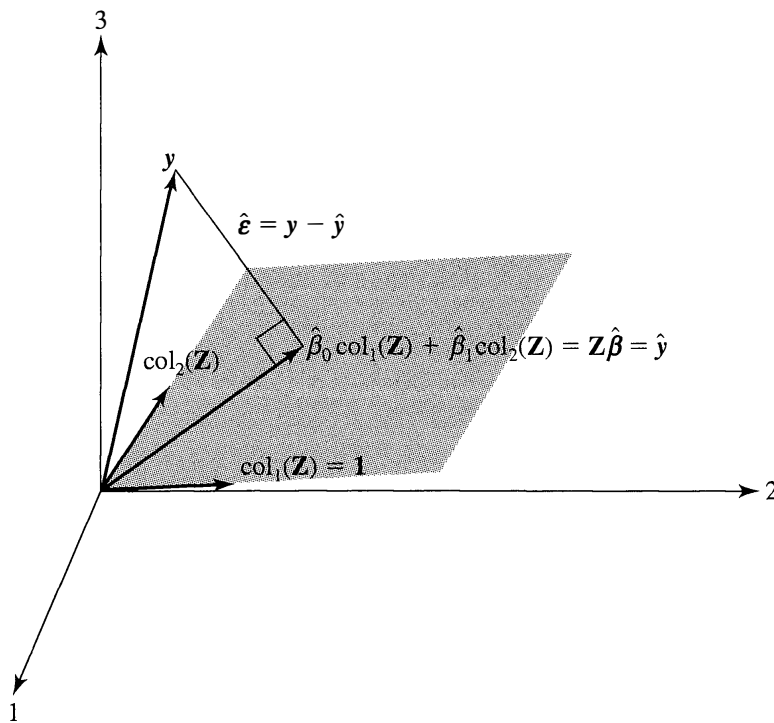
Figure 7.1 Least squares as a projection for n = 3, r = 1 .
