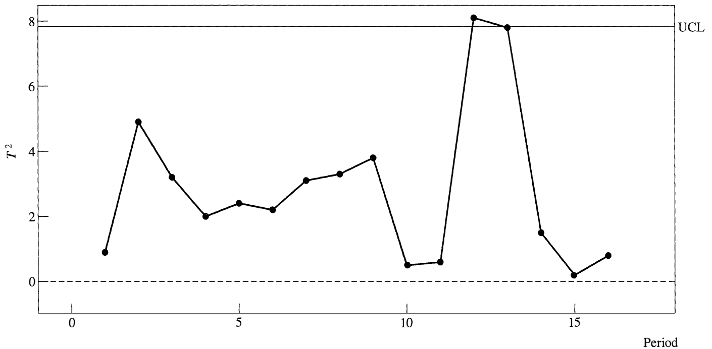
Figure 8.8 A T^2 -chart based on the last three principal components of overtime hours.
