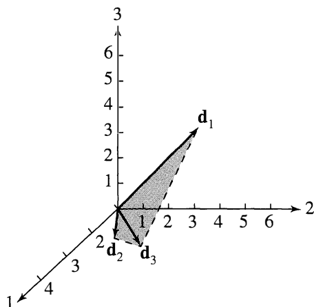
Figure 3.9 A case where the three-dimensional volume is zero ( |\mathbf{S}| = 0 ).
