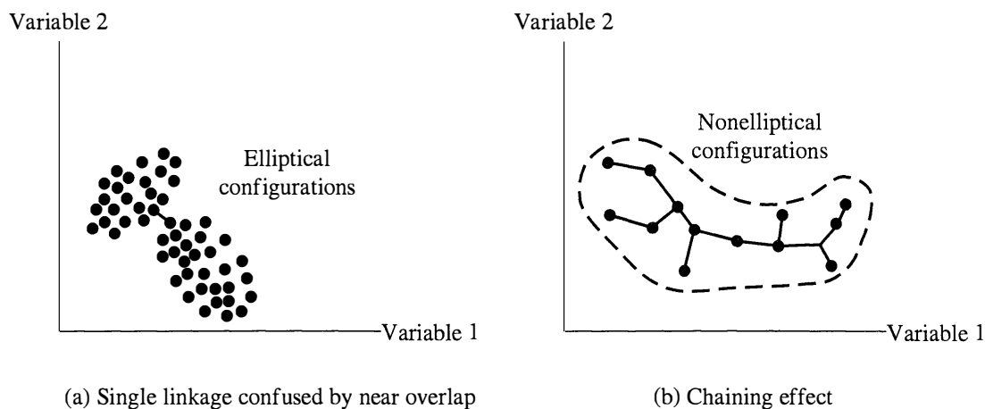
Figure 12.6 Single linkage clusters.
