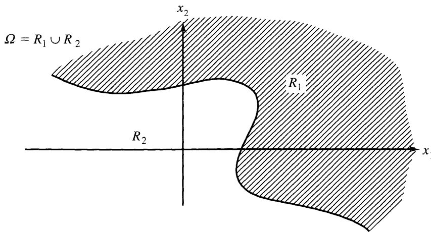
Figure 11.2 Classification regions for two populations.
