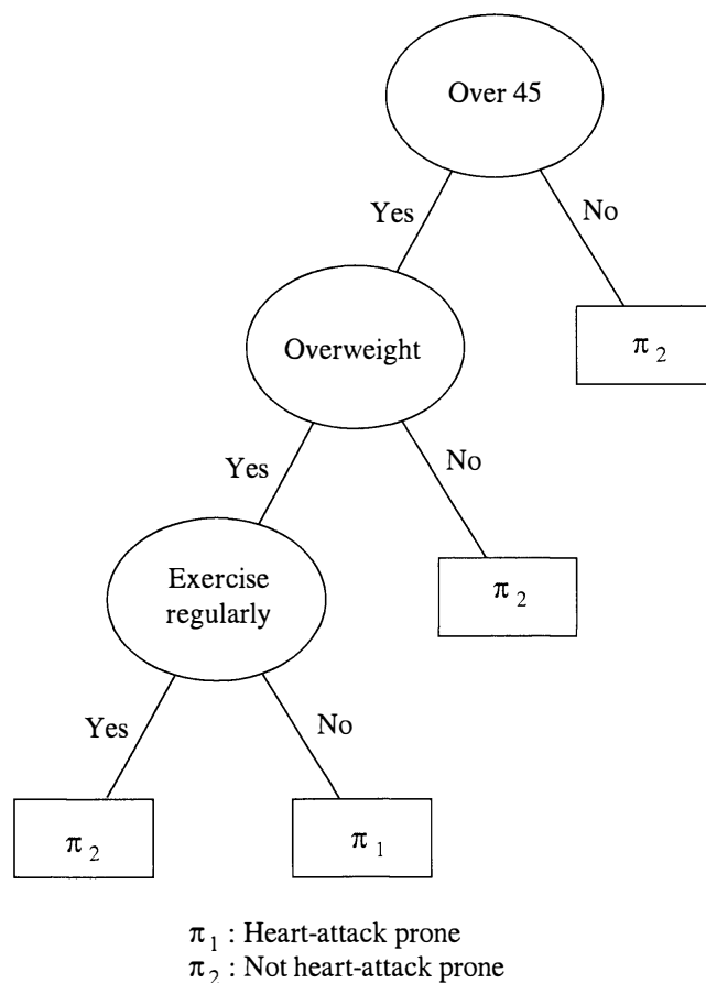
Figure 11.15 A classification tree.
