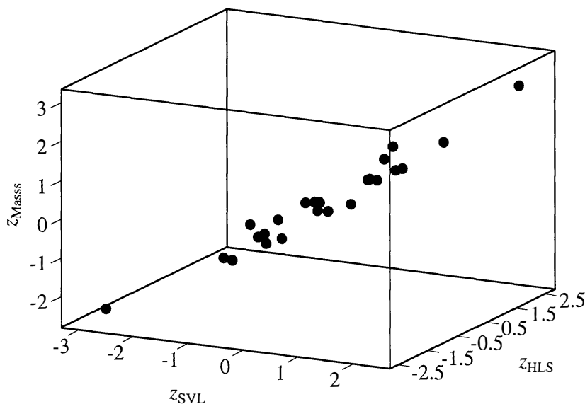
Figure 1.7 3D scatter plot of standardized lizard data.
