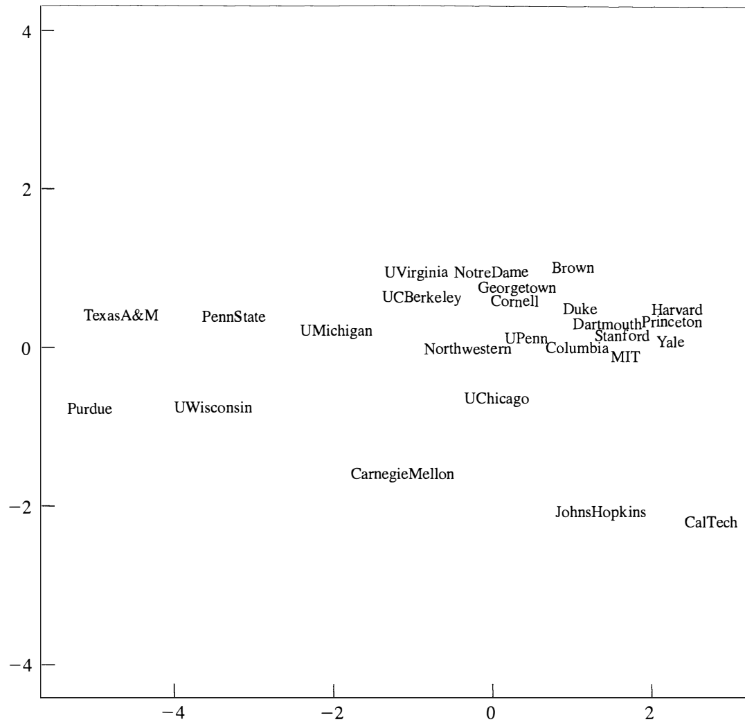
Figure 12.18 A two-dimensional representation of universities produced by metric multidimensional scaling.
