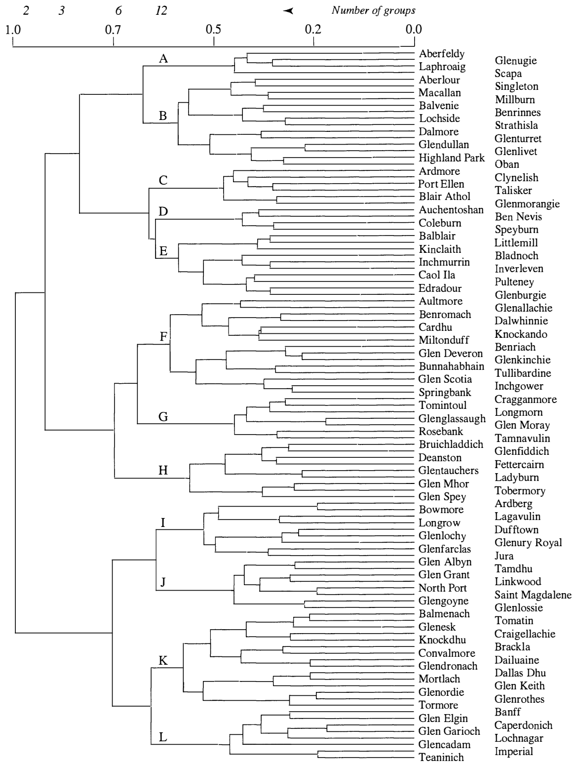
Figure 12.12 A dendrogram for similarities between 109 pure malt Scotch whiskies.
