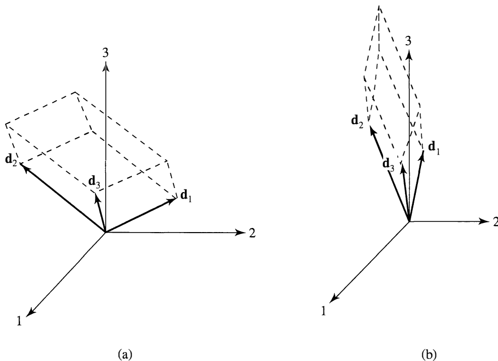
Figure 3.6 (a) “Large” generalized sample variance for p = 3 . (b) “Small” generalized sample variance for p = 3 .
