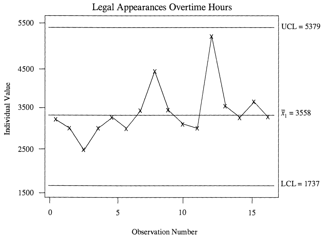
Figure 5.5 The \bar{X} -chart for x_1 = legal appearances overtime hours.
