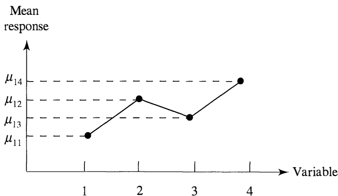
Figure 6.4 The population profile p = 4 .
