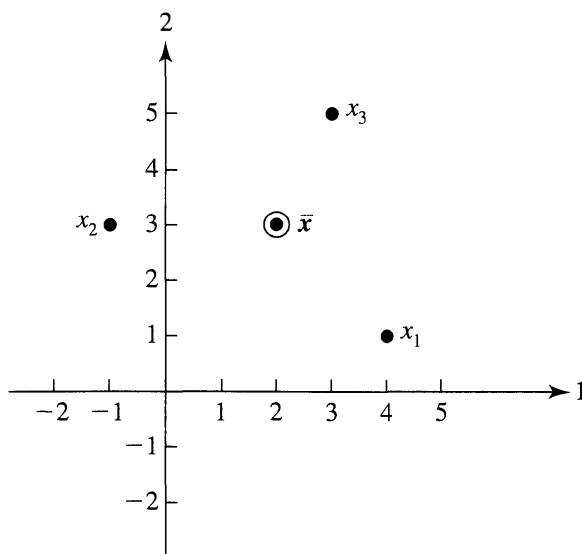
Figure 3.1 A plot of the data matrix \mathbf{X} as n = 3 points in p = 2 space.
