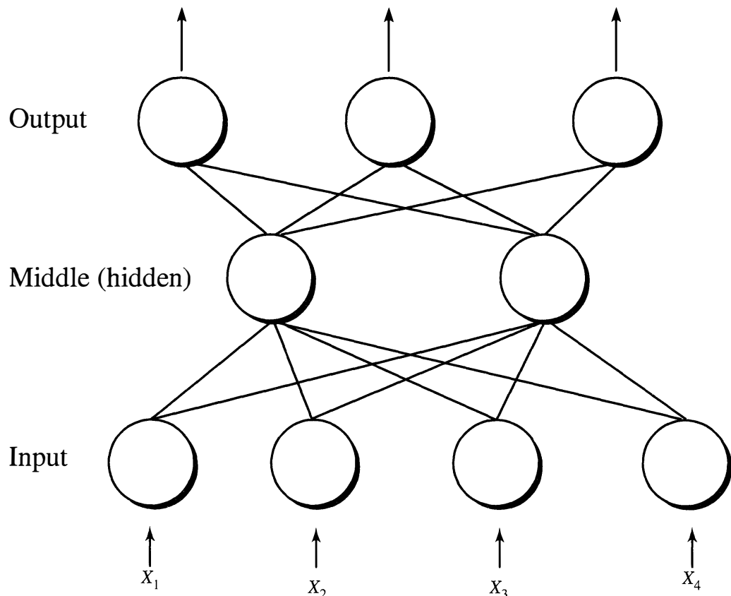
Figure 11.18 A neural network with one hidden layer.
