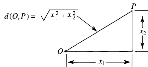
Figure 1.19 Distance given by the Pythagorean theorem.
