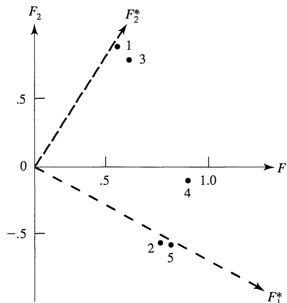
Figure 9.2 Factor rotation for hypothetical marketing data.
