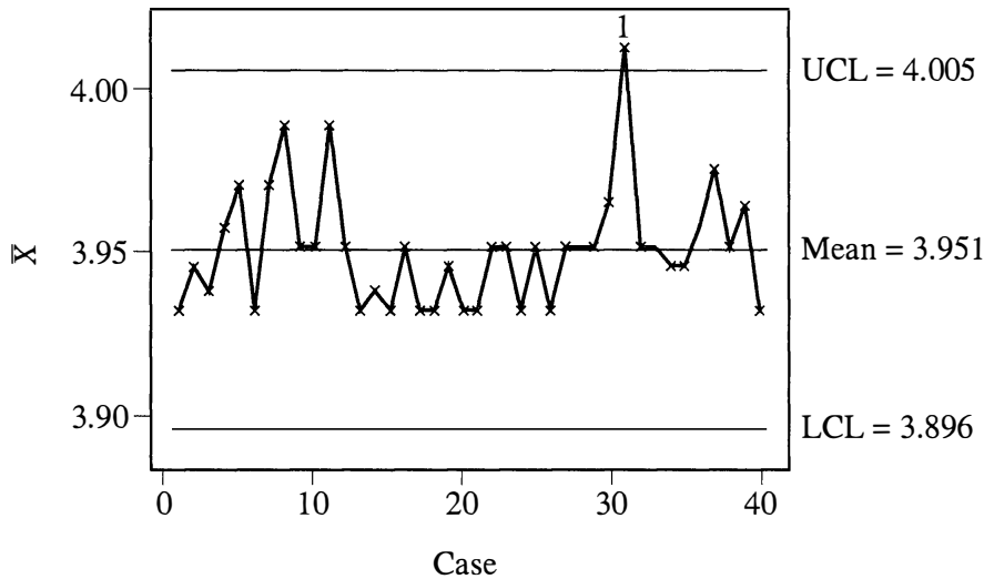
Figure 5.11 The univariate \bar{X} -chart for \ln(\text{gas flow}) .
