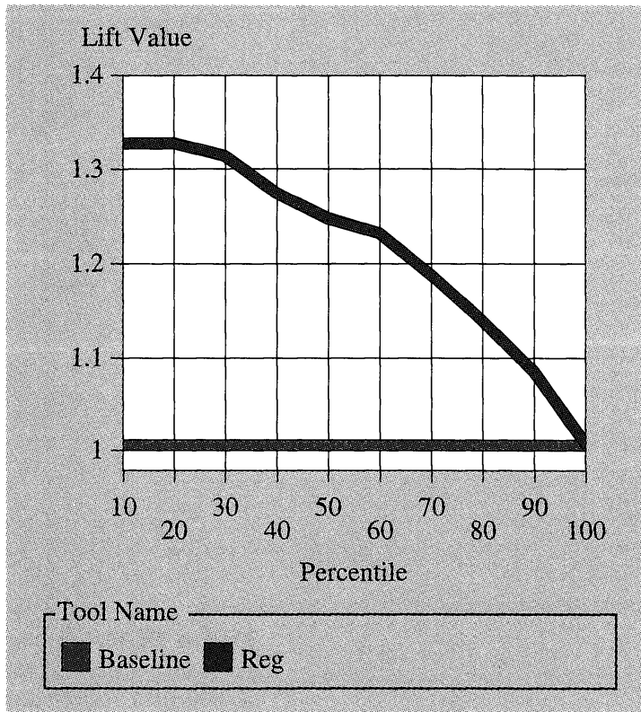
Figure 12.29 Cumulative lift chart for the logistic regression classifier.
