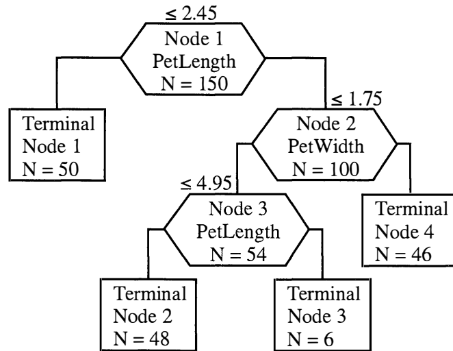
Figure 11.16 A classification tree for the Iris data.
