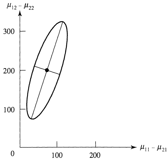
Figure 6.2 95% confidence ellipse for \boldsymbol{\mu}'_1 - \boldsymbol{\mu}'_2 = (\mu_{11} - \mu_{21}, \mu_{12} - \mu_{22}) .
