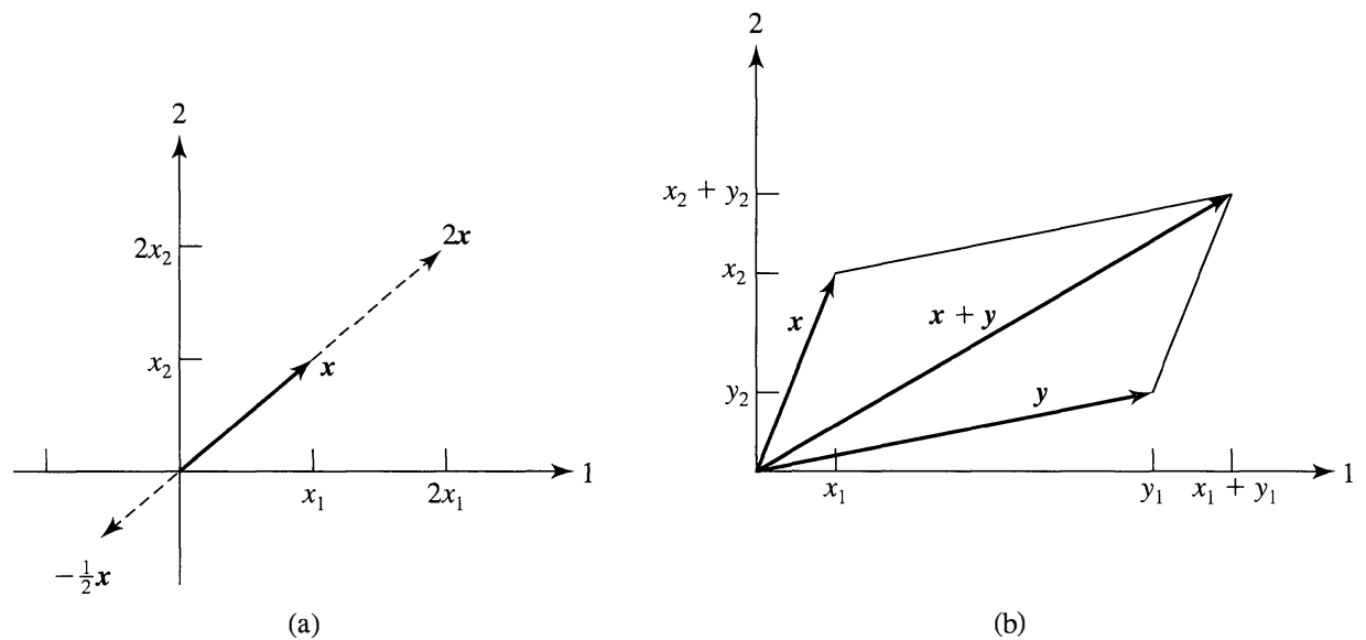
Figure 2.2 Scalar multiplication and vector addition.
