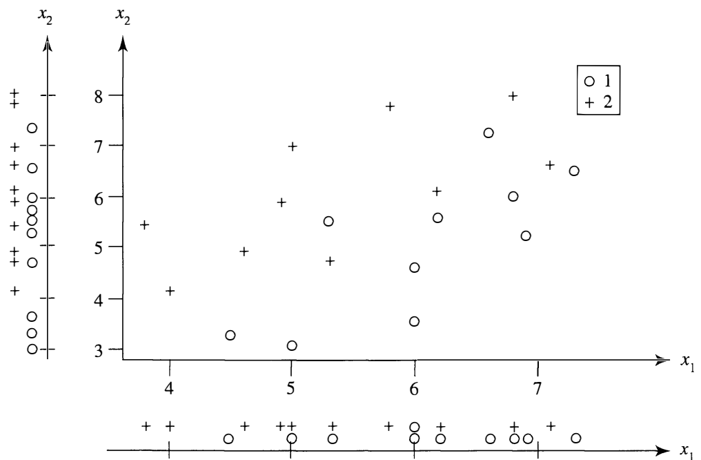
Figure 6.6 Scatter plots and marginal dot diagrams for the data from two groups.
