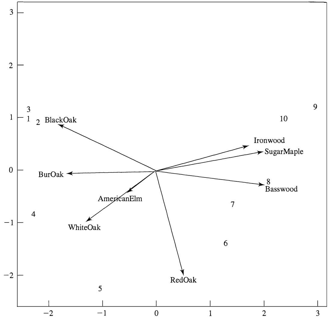
Figure 12.27 The biplot of the data on forests.
