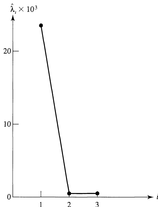
Figure 8.3 A scree plot for the turtle data.
