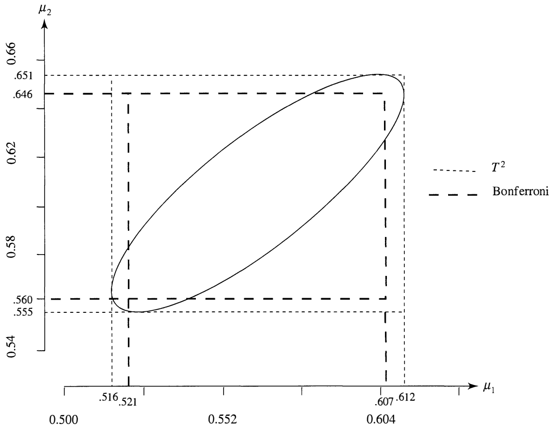
Figure 5.4 The 95% T^2 and 95% Bonferroni simultaneous confidence intervals for the component means—microwave radiation data.
