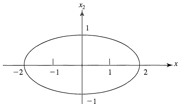
Figure 1.22 Ellipse of unit distance, \frac{x_1^2}{4} + \frac{x_2^2}{1} = 1 .
