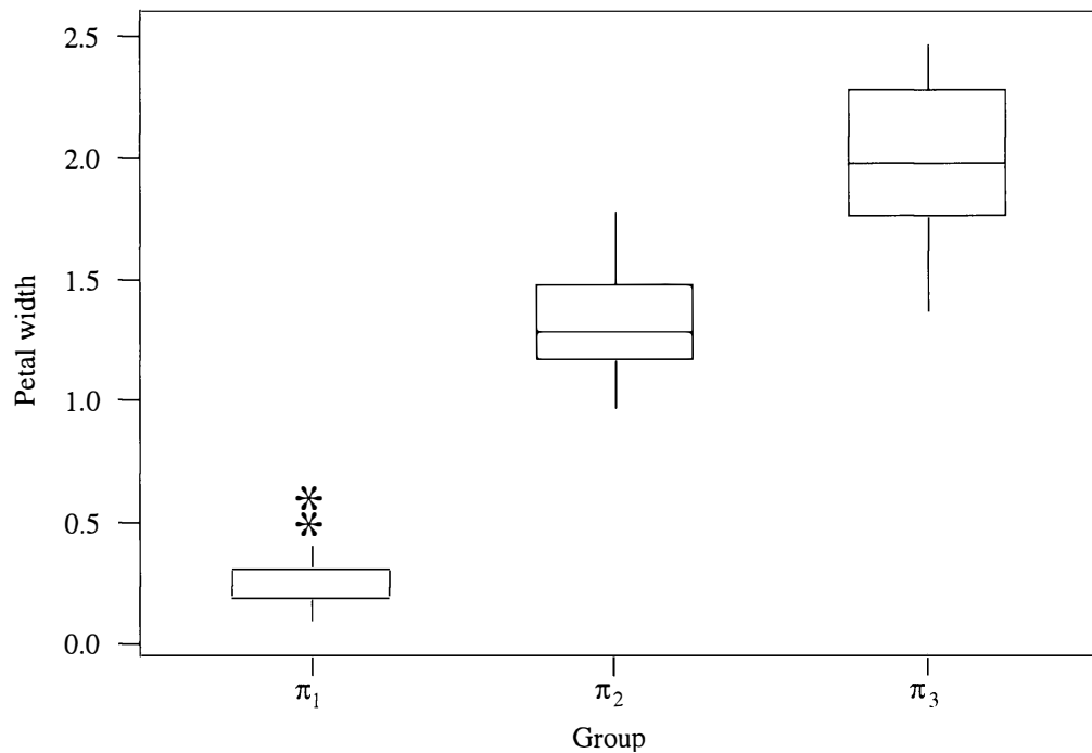
Figure 11.11 Box plots of petal width for the three species of iris.
