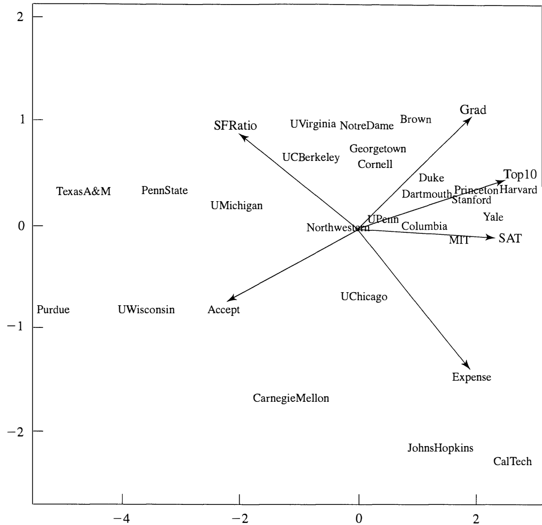
Figure 12.23 A biplot of the data on universities.
