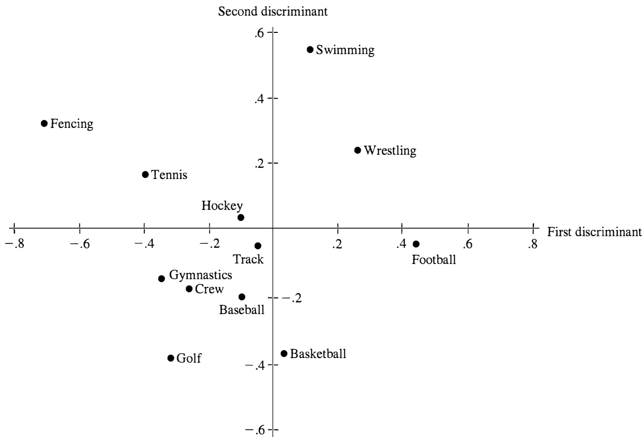
Figure 11.13 The discriminant means \bar{\mathbf{y}}' = [\bar{y}_1, \bar{y}_2] for each sport.
