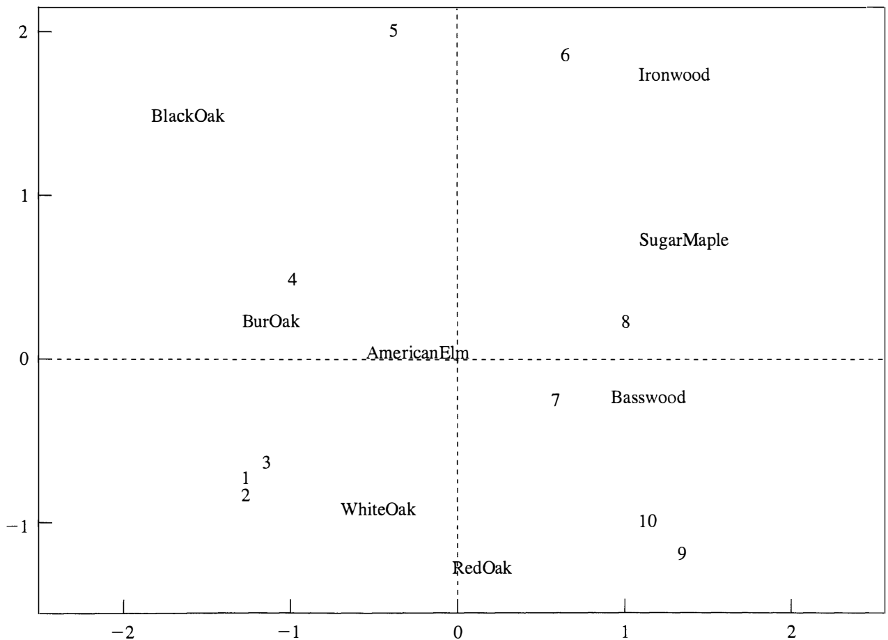
Figure 12.26 The correspondence analysis plot of the data on forests.
