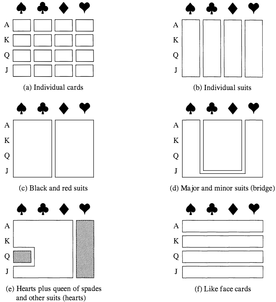
Figure 12.1 Grouping face cards.
