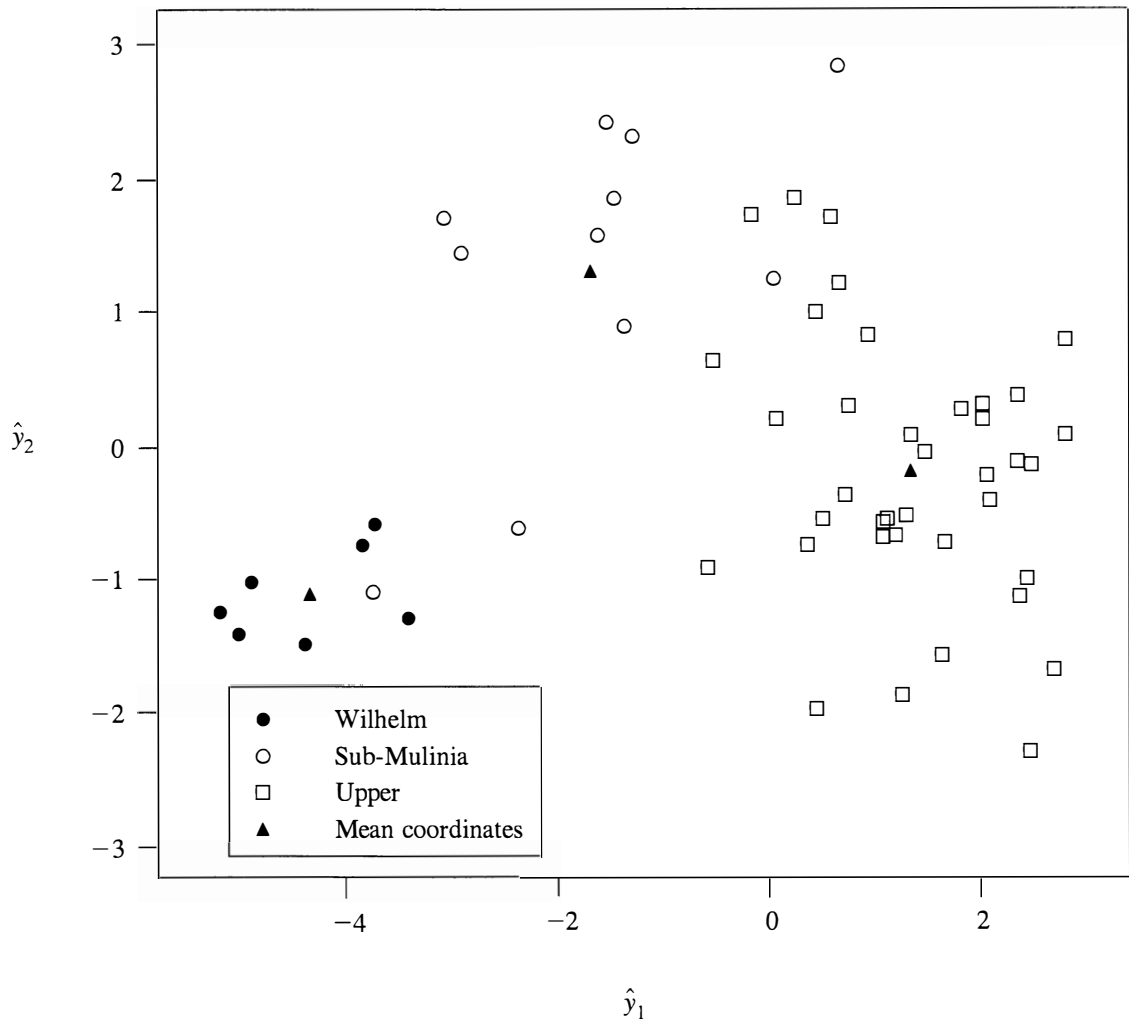
Figure 11.12 Crude-oil samples in discriminant space.
