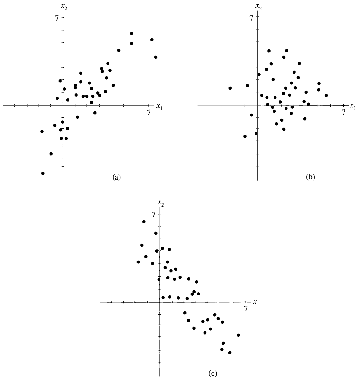
Figure 3.7 Scatter plots with three different orientations.
