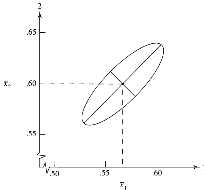
Figure 5.1 A 95% confidence ellipse for \boldsymbol{\mu} based on microwave-radiation data.
