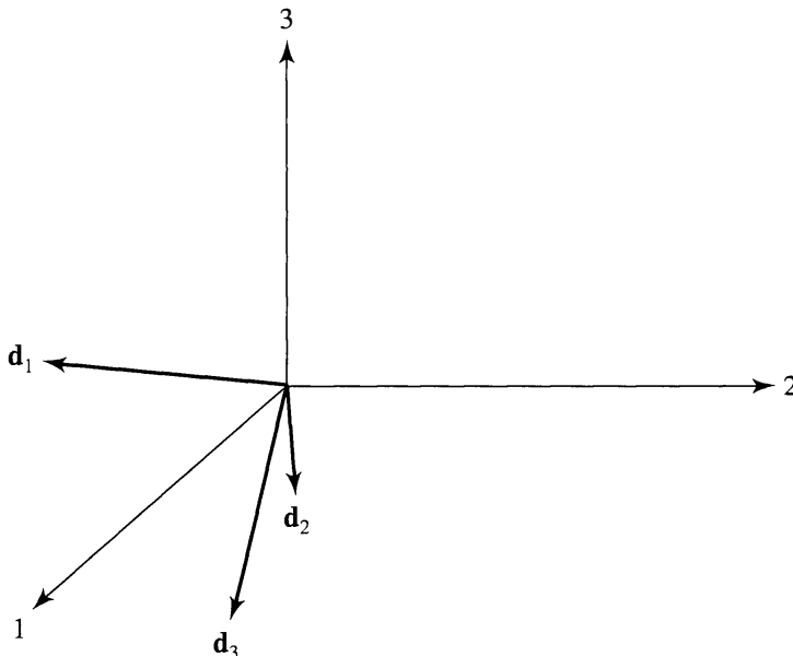
Figure 3.4 The deviation vectors \mathbf{d}_i from Figure 3.3.
