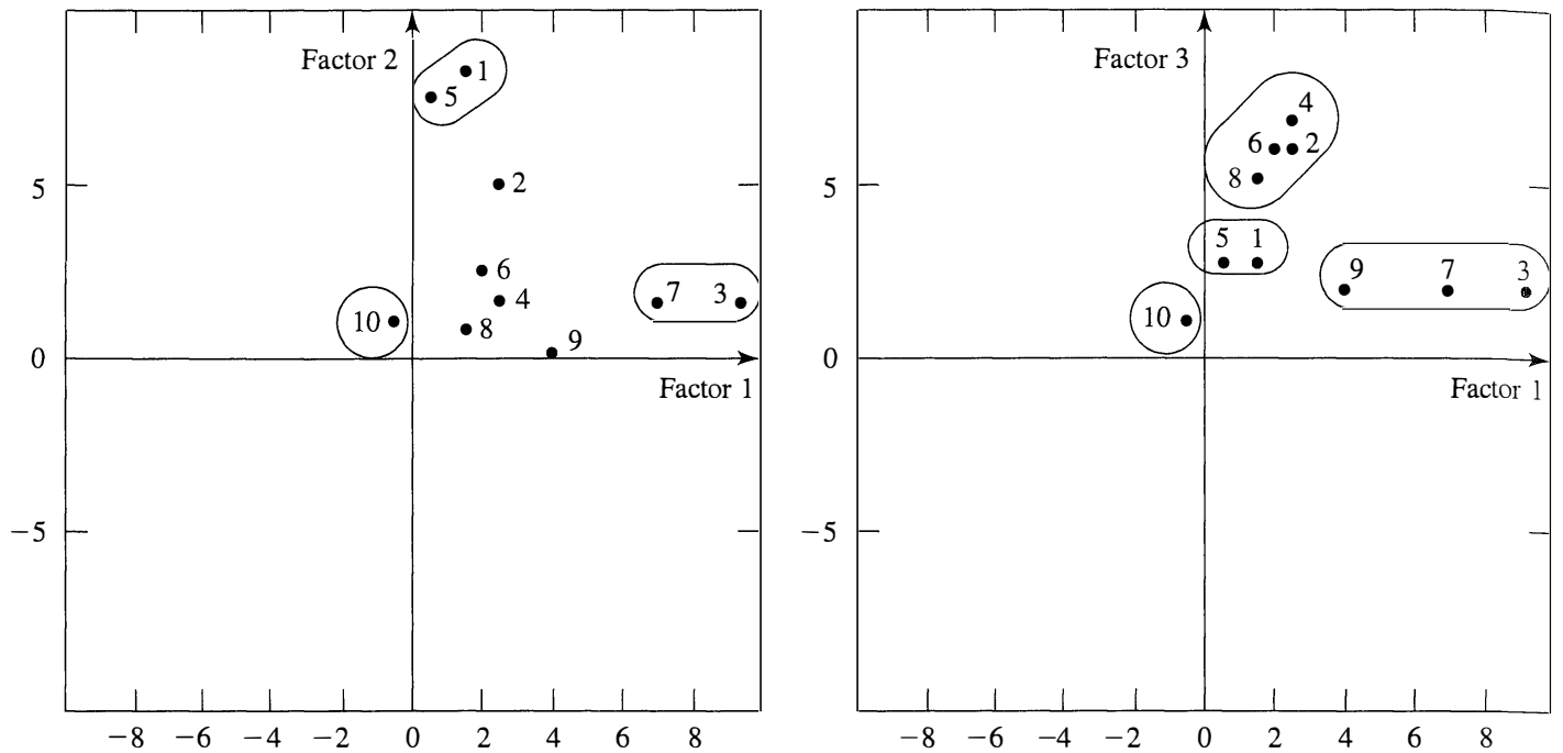
Figure 9.3 Rotated maximum likelihood loadings for factor pairs (1, 2) and (1, 3)—decathlon data. (The numbers in the figures correspond to variables.)
