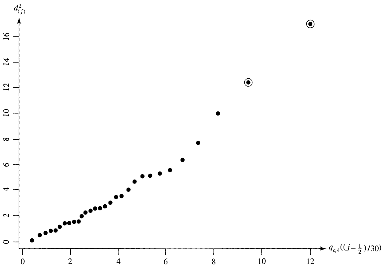
Figure 4.9 A chi-square plot for the data in Example 4.14.
