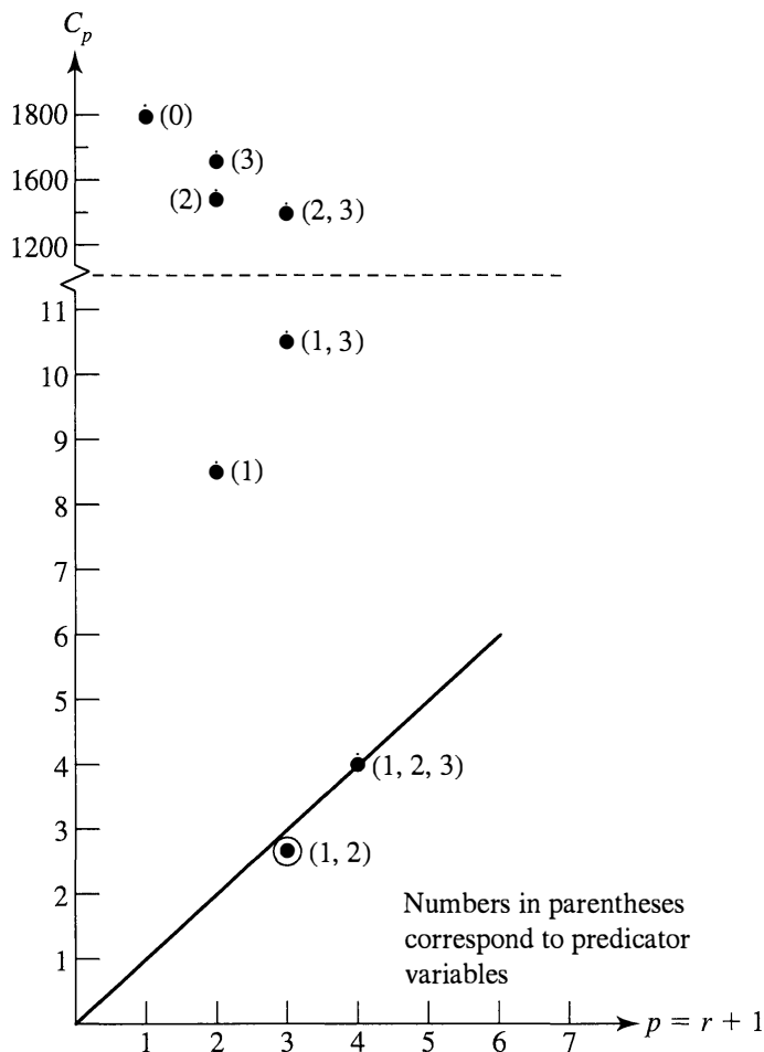
Figure 7.4 C_p plot for computer data from Example 7.6 with three predictor variables ( z_1 = orders, z_2 = add-delete count, z_3 = number of items; see the example and original source).
