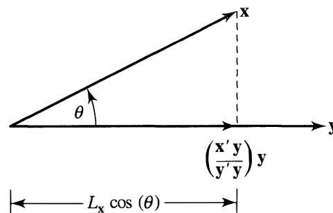
Figure 2.5 The projection of \mathbf{x} on \mathbf{y} .
