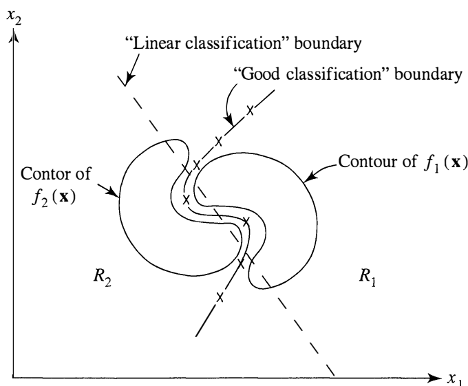
Figure 11.19 Two nonnormal populations for which linear discrimination is inappropriate.
