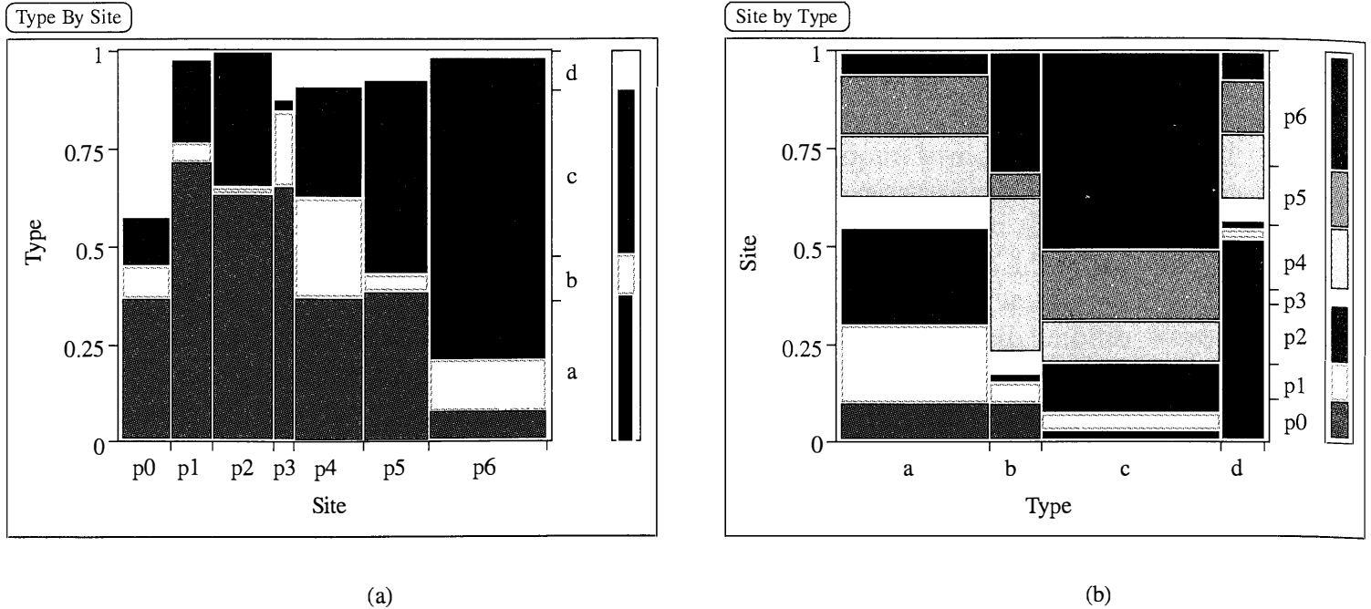
Figure 12.20 Site and pottery type profiles for the data in Table 12.8.
