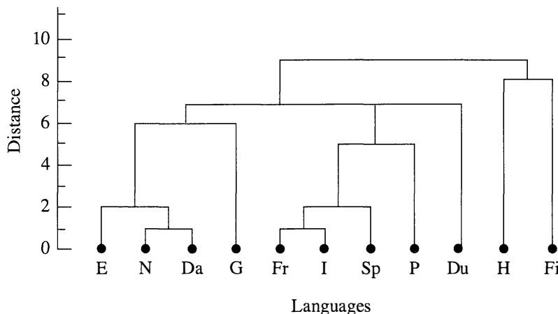
Figure 12.8 Complete linkage dendrogram for distances between numbers in 11 languages.
