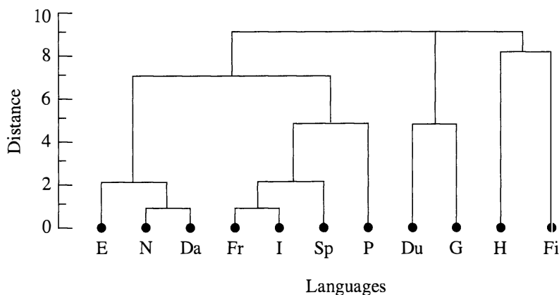
Figure 12.5 Single linkage dendrograms for distances between numbers in 11 languages.
