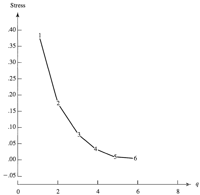
Figure 12.16 Stress function for distances between utilities.
