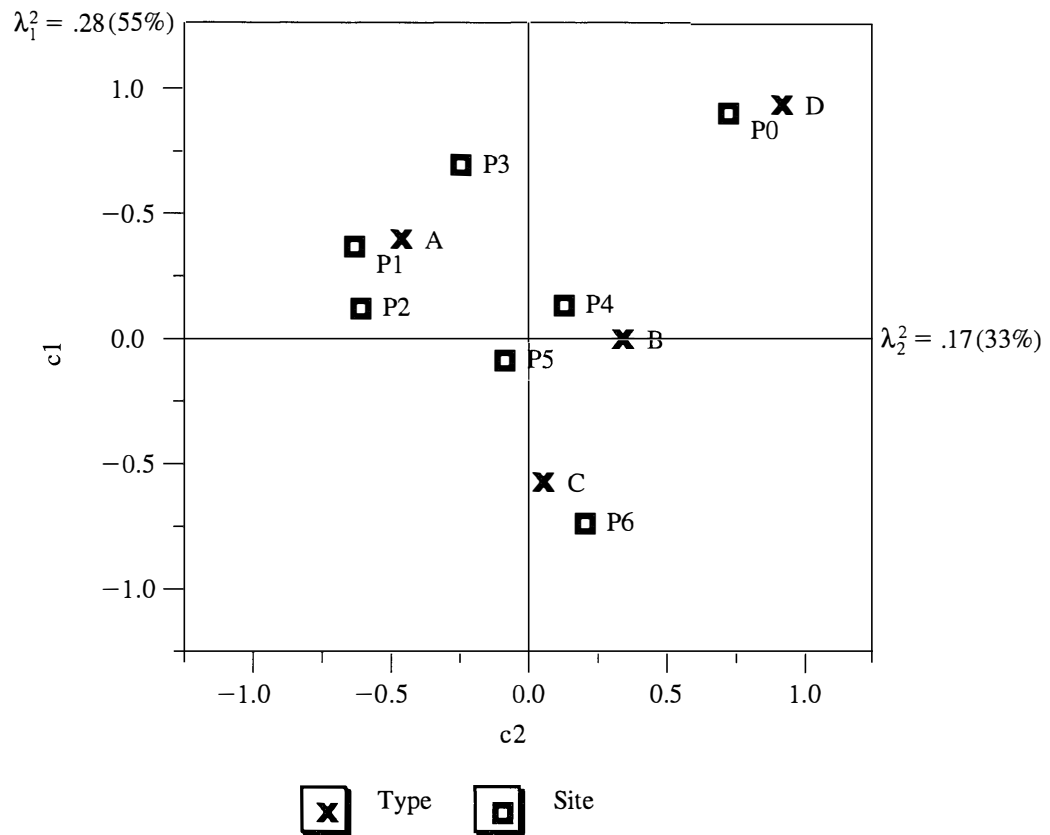
Figure 12.21 A correspondence analysis plot of the pottery type–site data.
