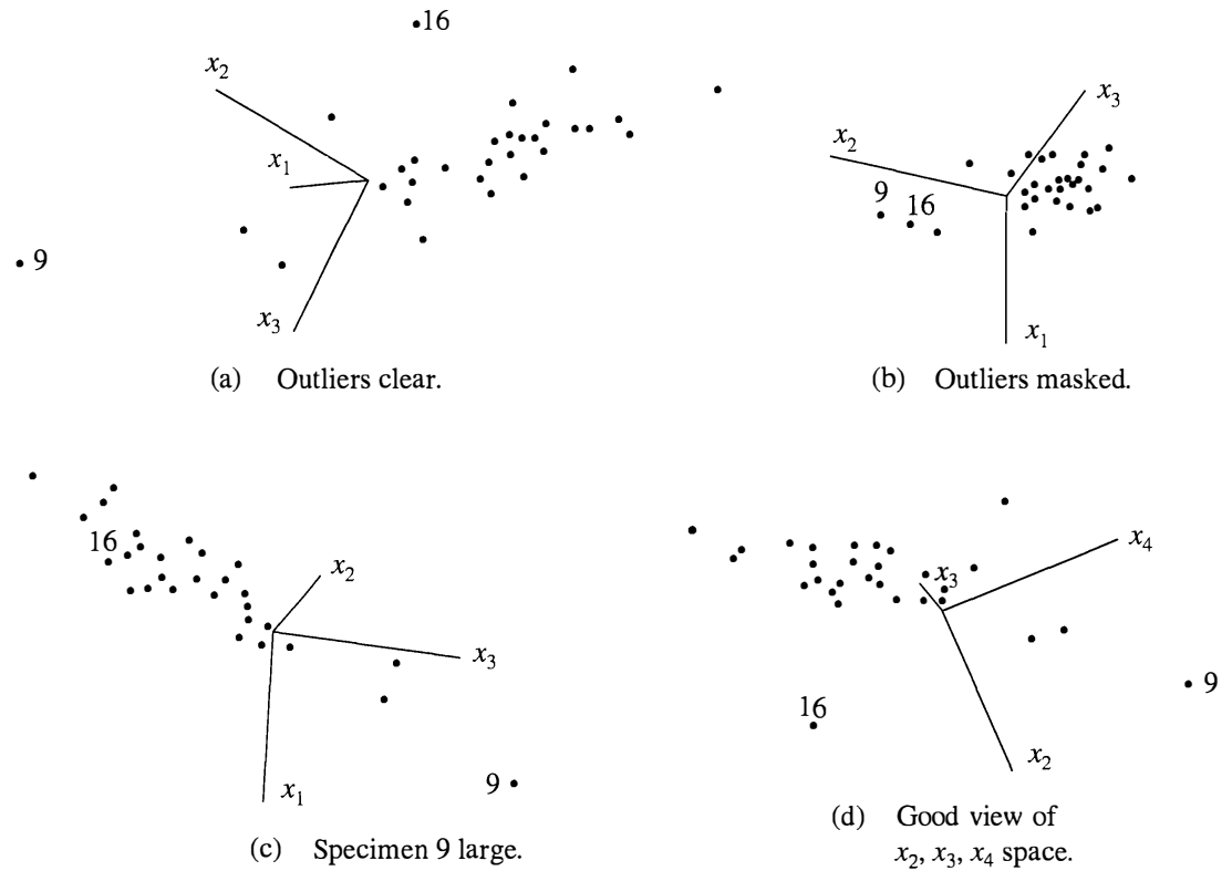
Figure 1.12 Three-dimensional perspectives for the lumber stiffness data.
