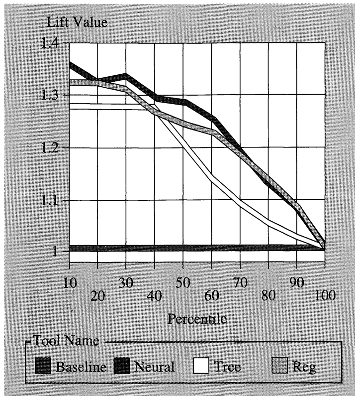
Figure 12.30 Cumulative lift charts for neural network, classification tree, and logistic regression tools.
