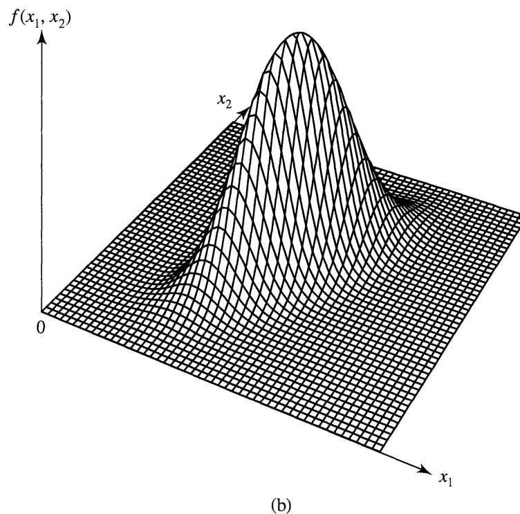
Figure 4.2 Two bivariate normal distributions. (a) \sigma_{11} = \sigma_{22} and \rho_{12} = 0 . (b) \sigma_{11} = \sigma_{22} and \rho_{12} = .75 .
