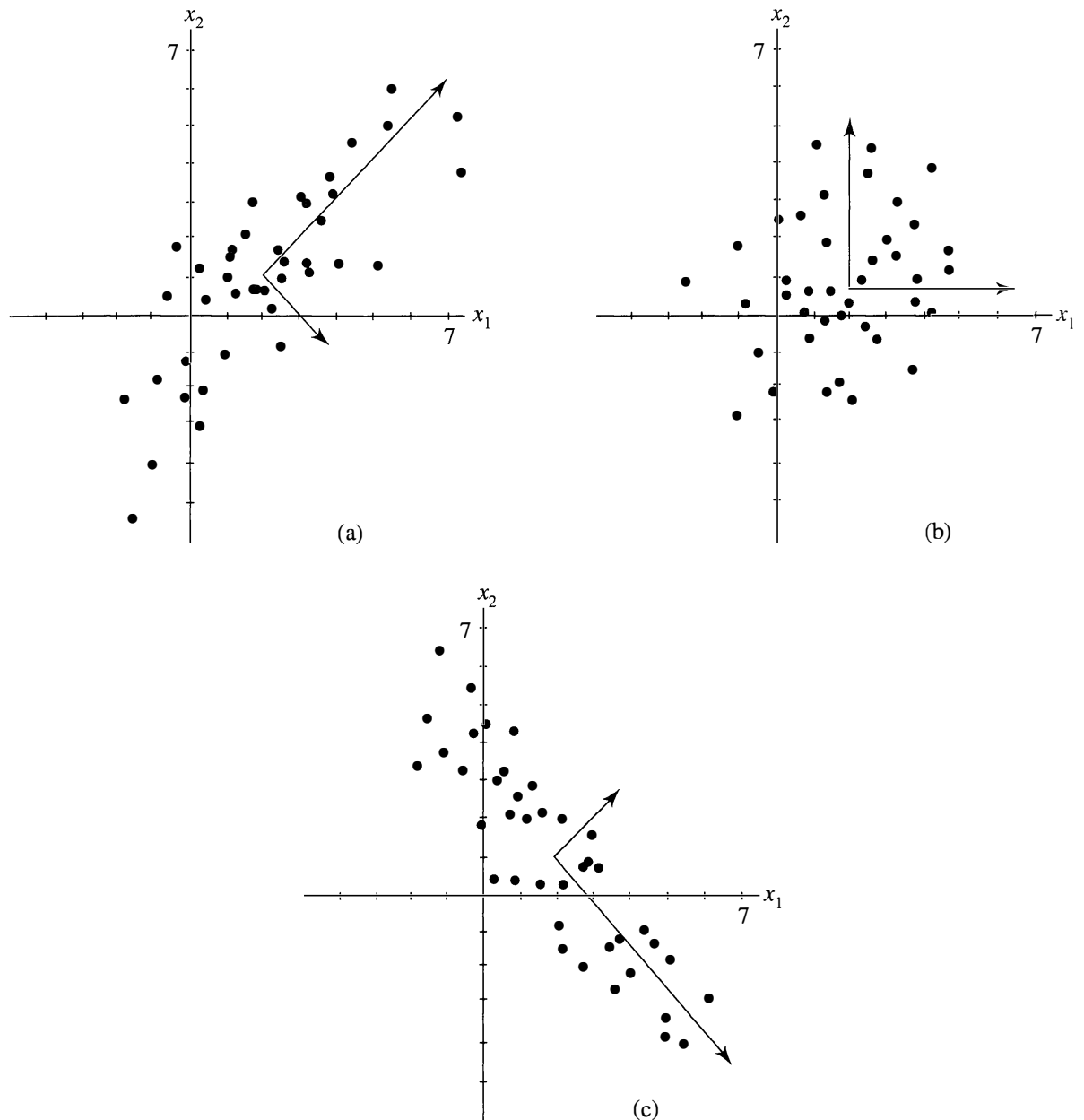
Figure 3.8 Axes of the mean-centered 95 percent ellipses for the scatter plots in Figure 3.7.
