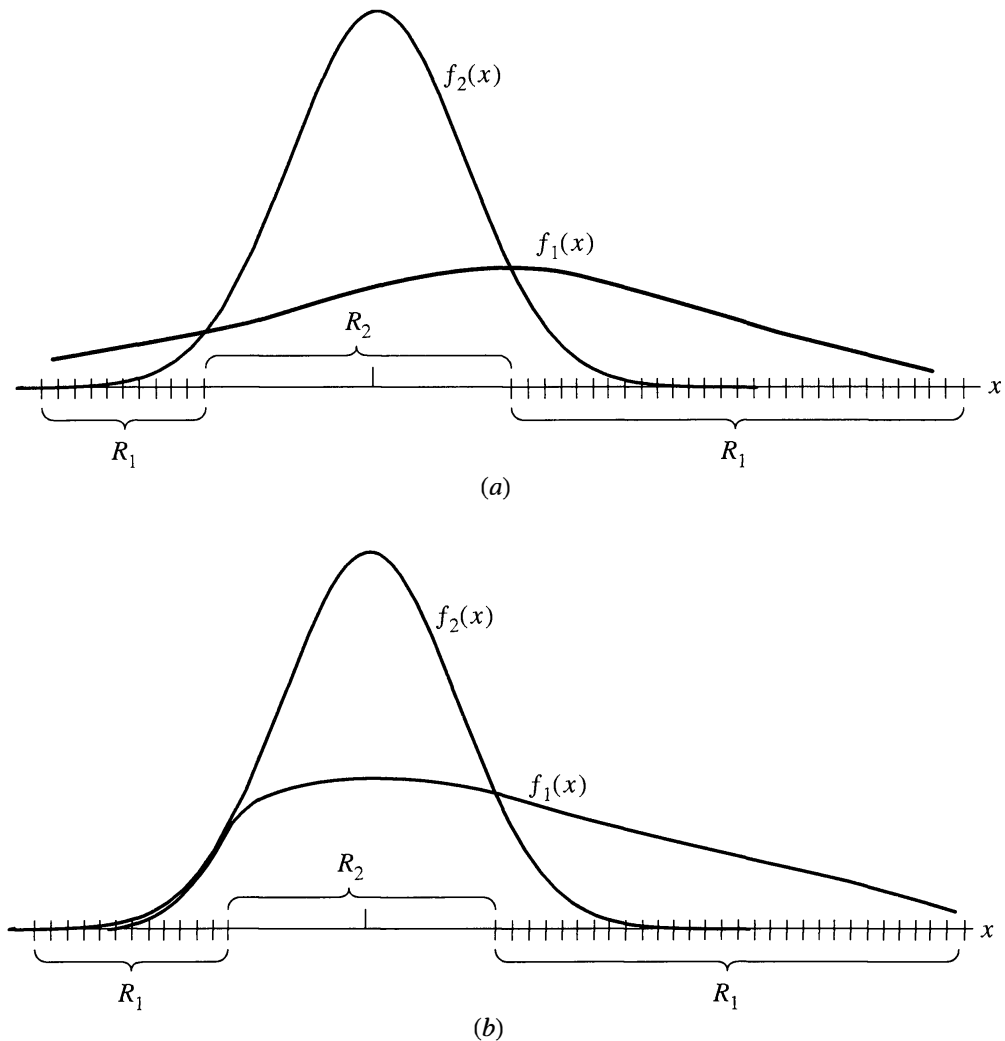
Figure 11.5 Quadratic rules for (a) two normal distribution with unequal variances and (b) two distributions, one of which is nonnormal—rule not appropriate.
