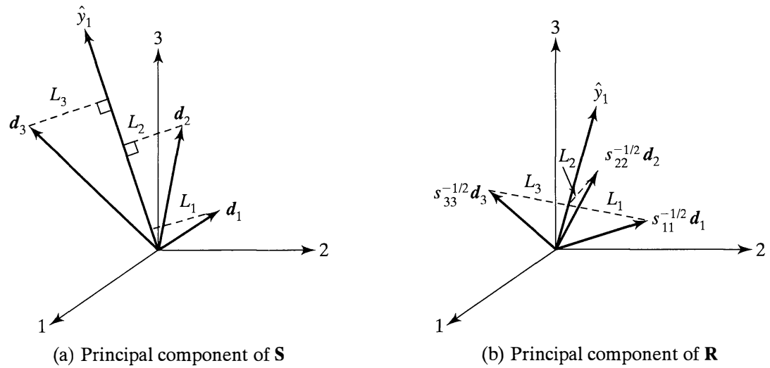
Figure 8.11 The first sample principal component, \hat{y}_1 , minimizes the sum of the squares of the distances, L_i^2 , from the deviation vectors, \mathbf{d}_i' = [x_{1i} - \bar{x}_i, x_{2i} - \bar{x}_i, \dots, x_{ni} - \bar{x}_i] , to a line.
