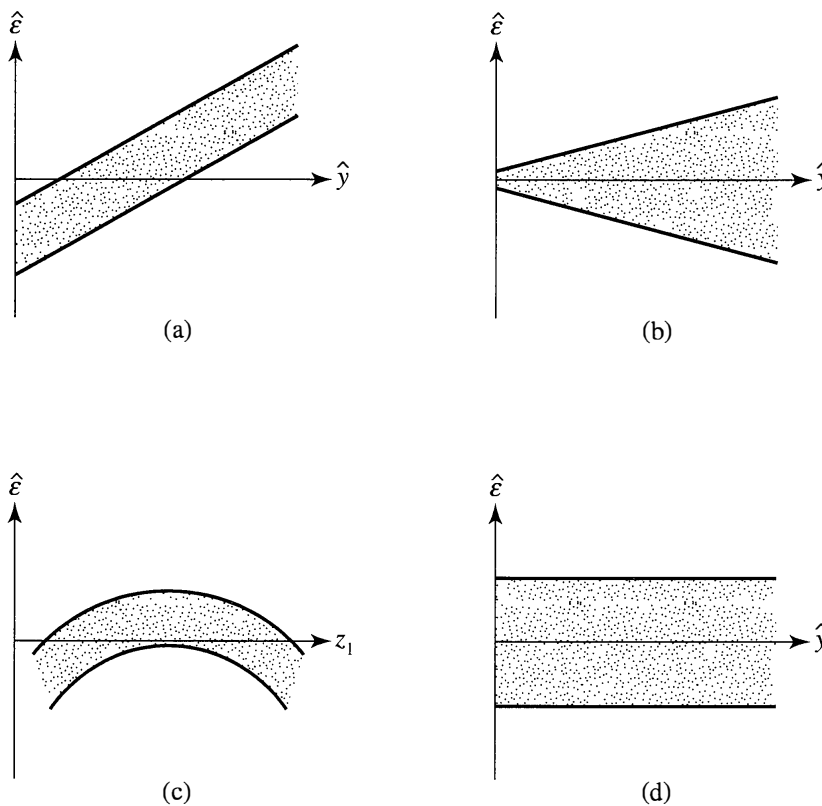
Figure 7.2 Residual plots.
