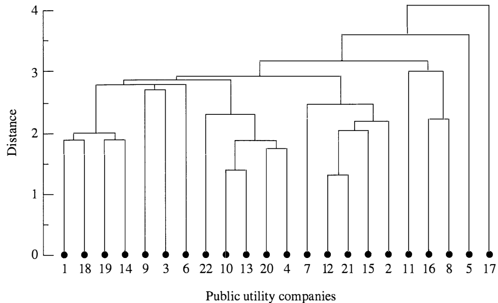
Figure 12.11 Average linkage dendrogram for distances between 22 public utility companies.
