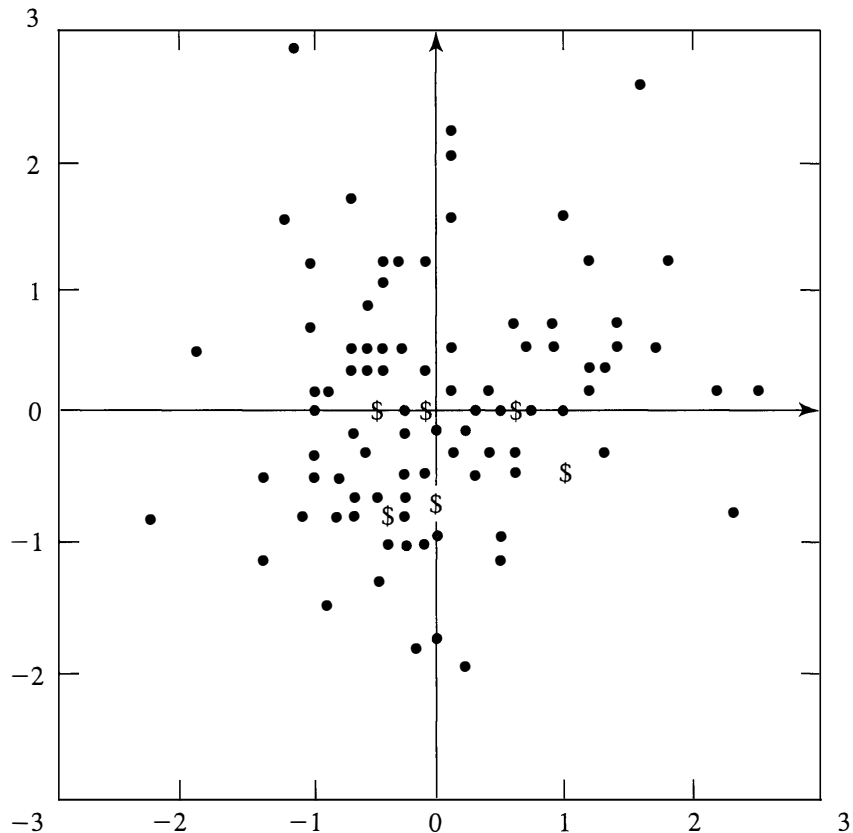
Figure 9.4 Factor scores using (9-58) for factors 1 and 2 of the stock-price data (maximum likelihood estimates of the factor loadings).
