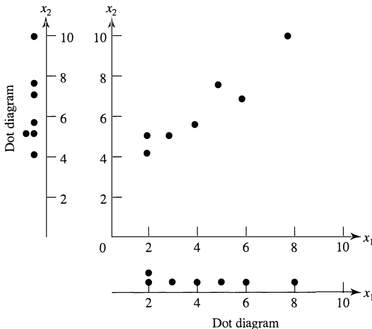
Figure 1.1 A scatter plot and marginal dot diagrams.
