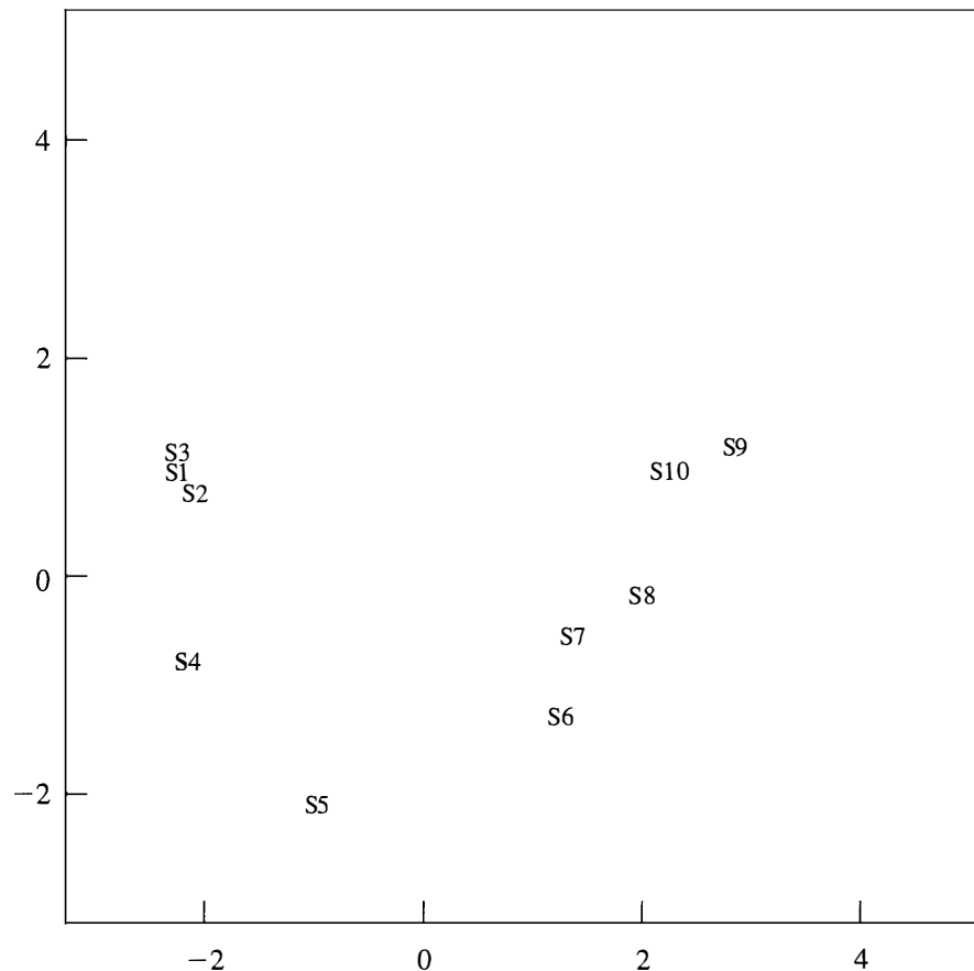
Figure 12.24 Metric multidimensional scaling of the data on forests.
