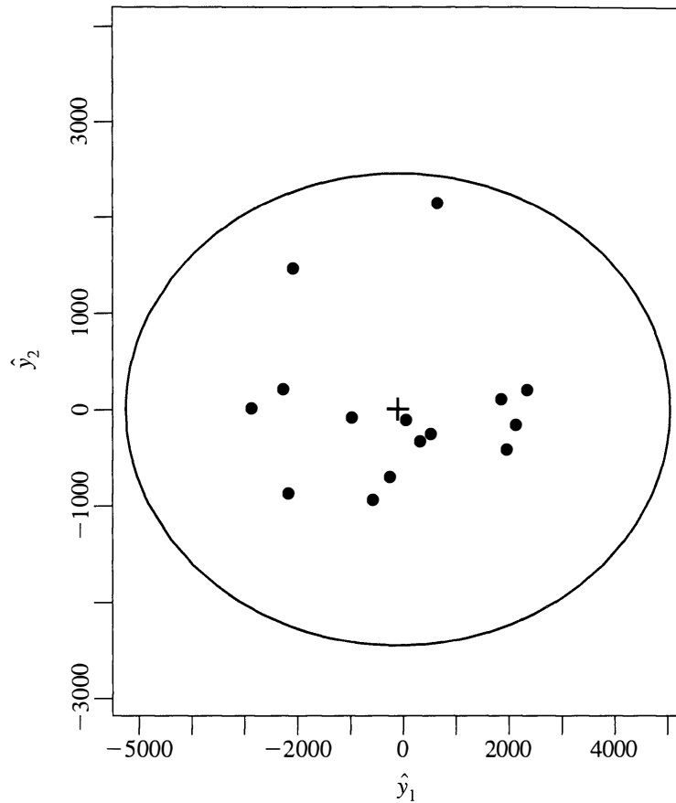
Figure 8.9 A 99% ellipse format chart for the first two principal components of future overtime.
