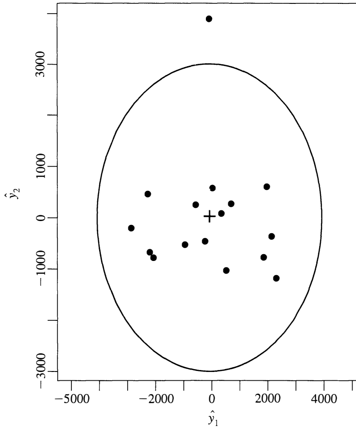
Figure 8.7 The 95% control ellipse based on the first two principal components of overtime hours.
