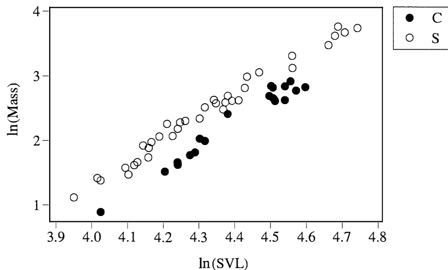
Figure 6.7 Scatter plot of \ln(\text{Mass}) versus \ln(\text{SVL}) for the lizard data in Table 6.7.
