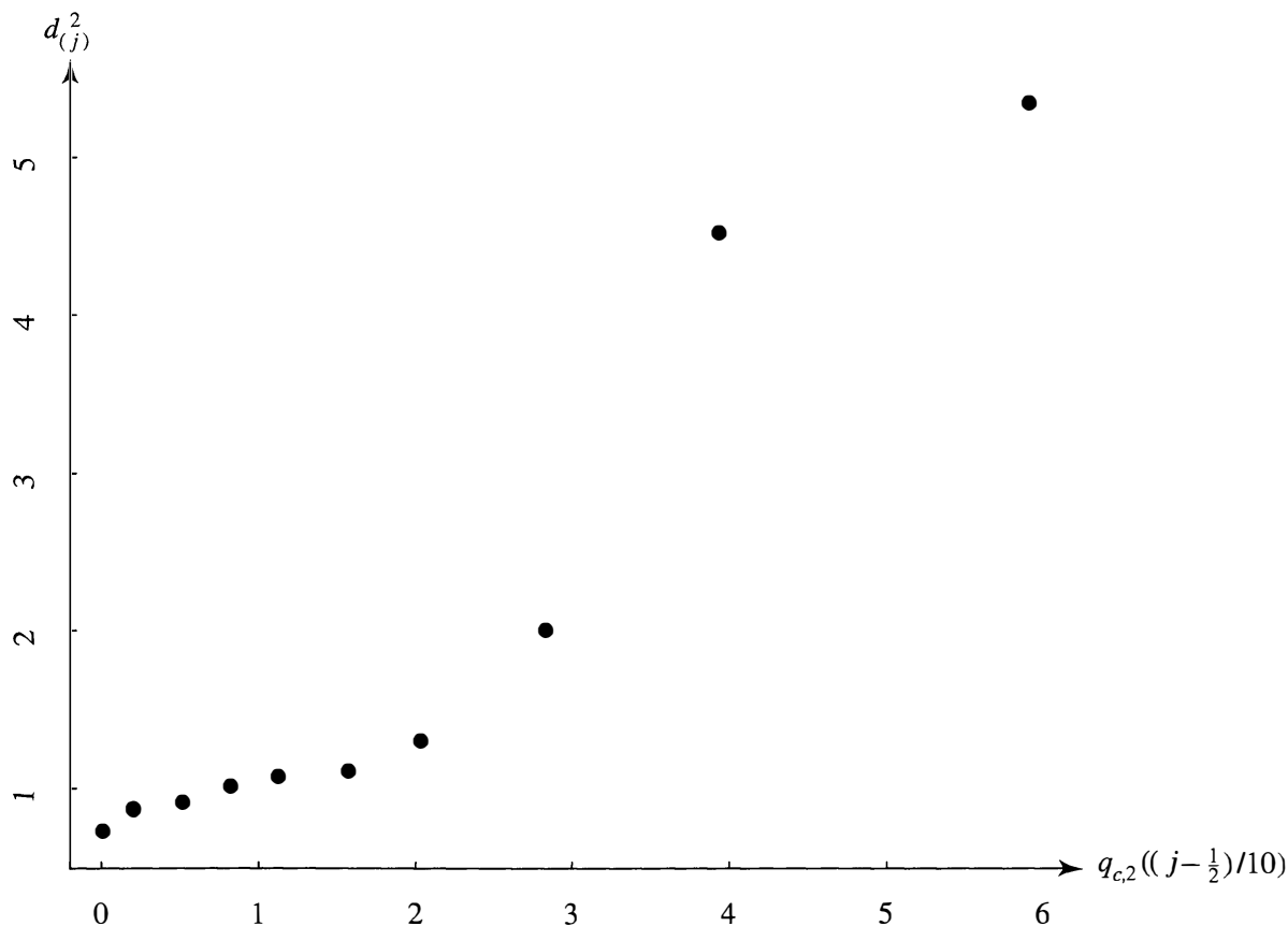
Figure 4.7 A chi-square plot of the ordered distances in Example 4.13.
