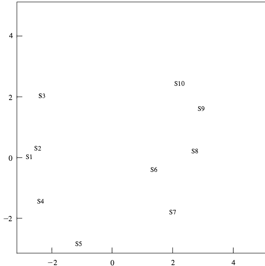
Figure 12.25 Nonmetric multidimensional scaling of the data on forests.
