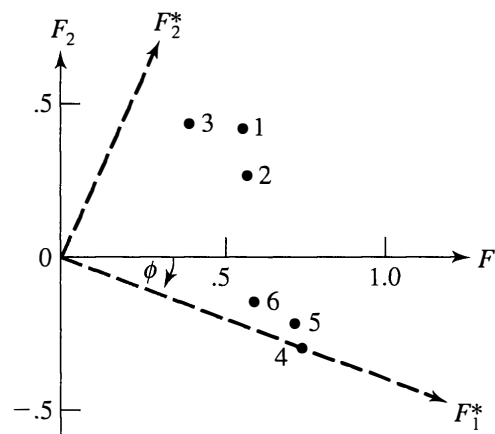
Figure 9.1 Factor rotation for test scores.
