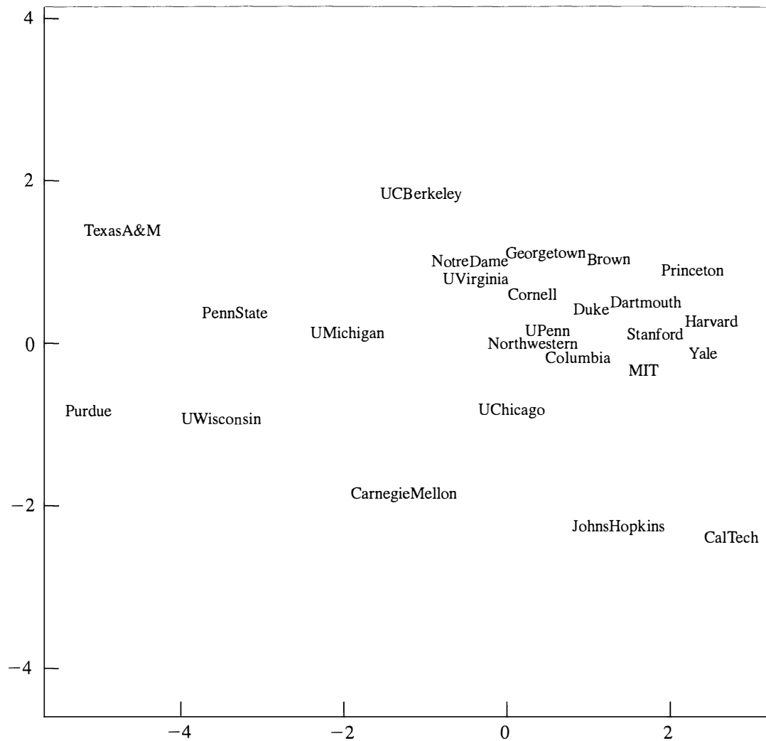
Figure 12.19 A two-dimensional representation of universities produced by nonmetric multidimensional scaling.
