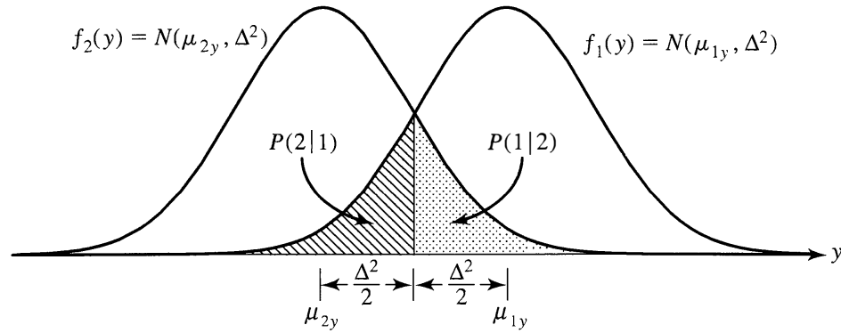
Figure 11.6 The misclassification probabilities based on Y .
