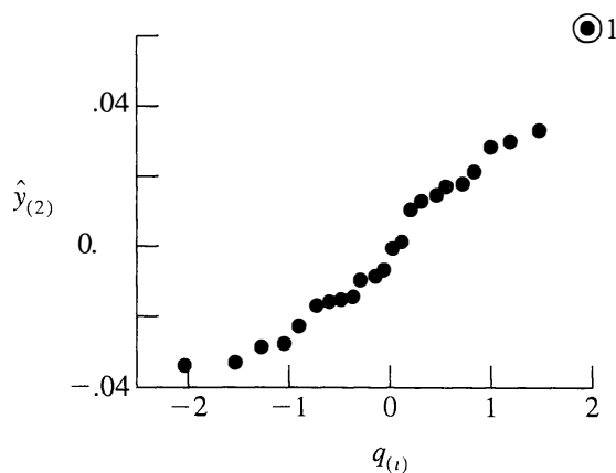
Figure 8.5 A Q-Q plot for the second principal component \hat{y}_2 from the data on male turtles.
