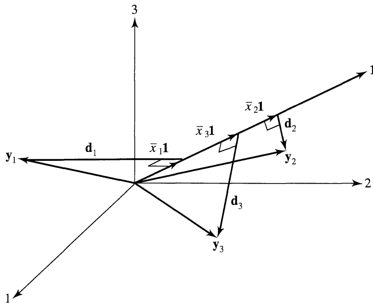
Figure 3.3 The decomposition of \mathbf{y}_i into a mean component \bar{x}_i\mathbf{1} and a deviation component \mathbf{d}_i = \mathbf{y}_i - \bar{x}_i\mathbf{1} , i = 1, 2, 3 .
