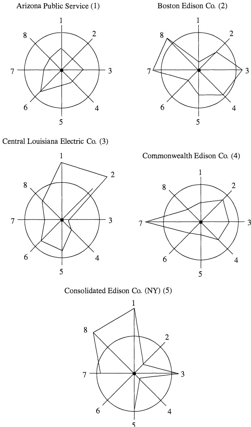
Figure 1.16 Stars for the first five public utilities.
