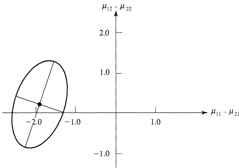
Figure 6.1 95% confidence ellipse for \boldsymbol{\mu}_1 - \boldsymbol{\mu}_2 .
