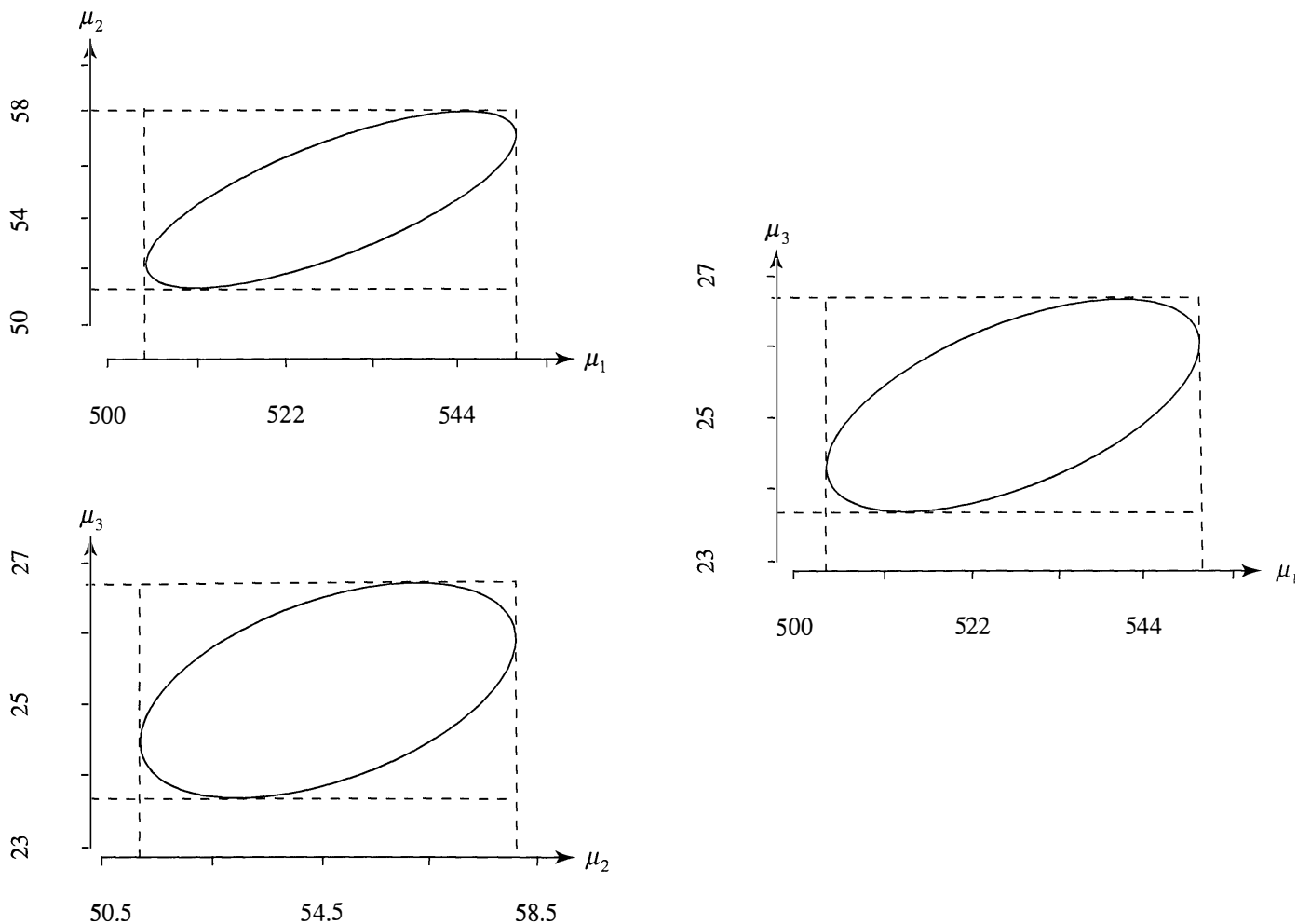
Figure 5.3 95% confidence ellipses for pairs of means and the simultaneous T^2 -intervals—college test data.
