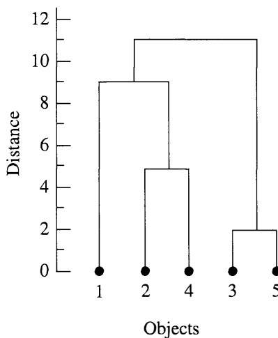
Figure 12.7 Complete linkage dendrogram for distances between five objects.
