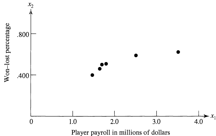
Figure 1.4 Salaries and won–lost percentage from Table 1.1.
