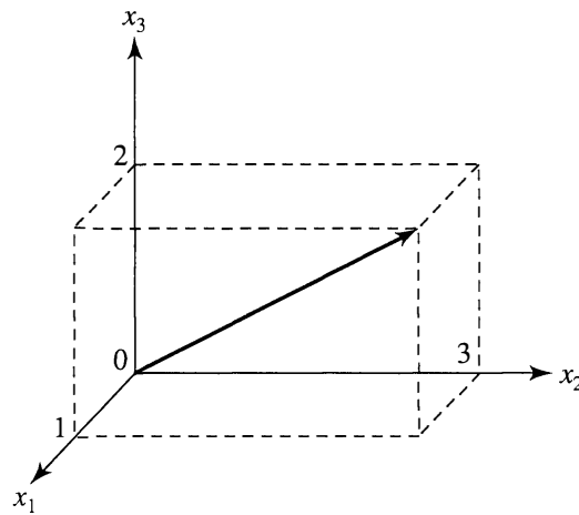
Figure 2.1 The vector \mathbf{x}' = [1, 3, 2] .
