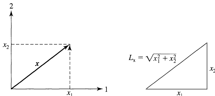
Figure 2.3 Length of \mathbf{x} = \sqrt{x_1^2 + x_2^2} .
