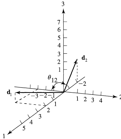
Figure 3.5 The deviation vectors \mathbf{d}_1 and \mathbf{d}_2 .
