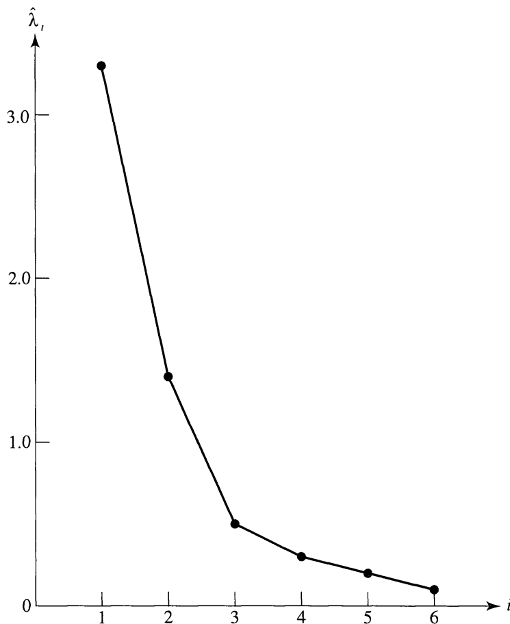
Figure 8.2 A scree plot.
