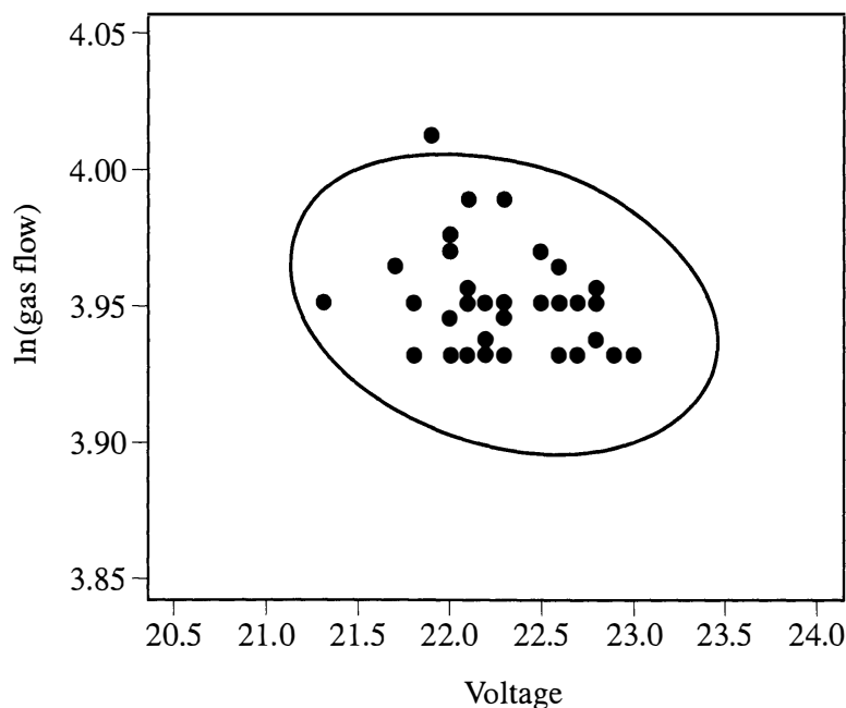
Figure 5.10 The 99% quality control ellipse for \ln(\text{gas flow}) and voltage.
